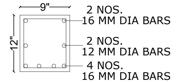
SEC. OF CORRIDOR R.C.C. DOWN BEAM
