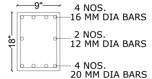
SEC. OF CLASSROOM R.C.C. DOWN BEAM
