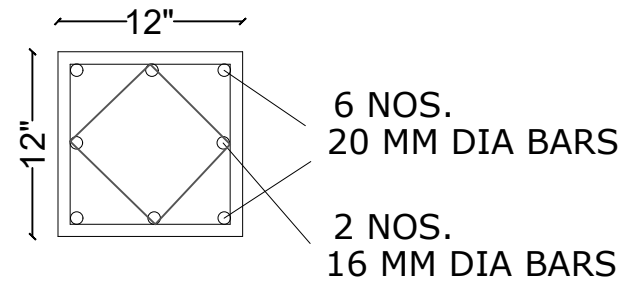
PLAN OF R.C.C COLUMN 12" X 12"
