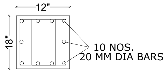
PLAN OF R.C.C COLUMN 12" X 18"
