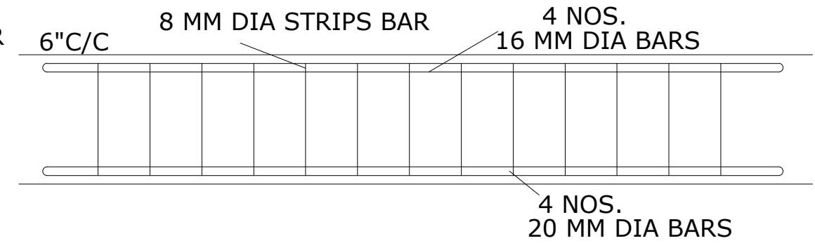
FRONT SEC. OF R.C.C. PLINTH BEAM
