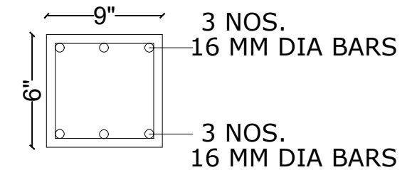
SEC. OF R.C.C. BEAM AT DOOR LVL
