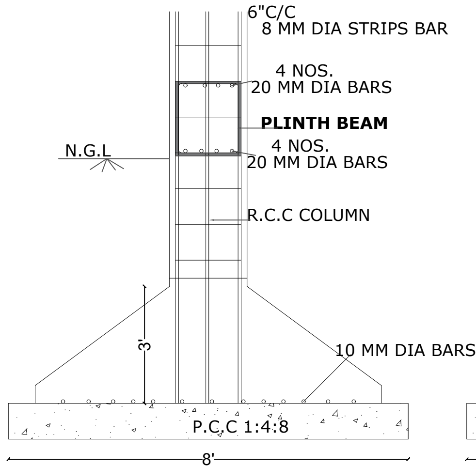
FOOTING DETAIL R.C.C COLUMN 12" X 18"
