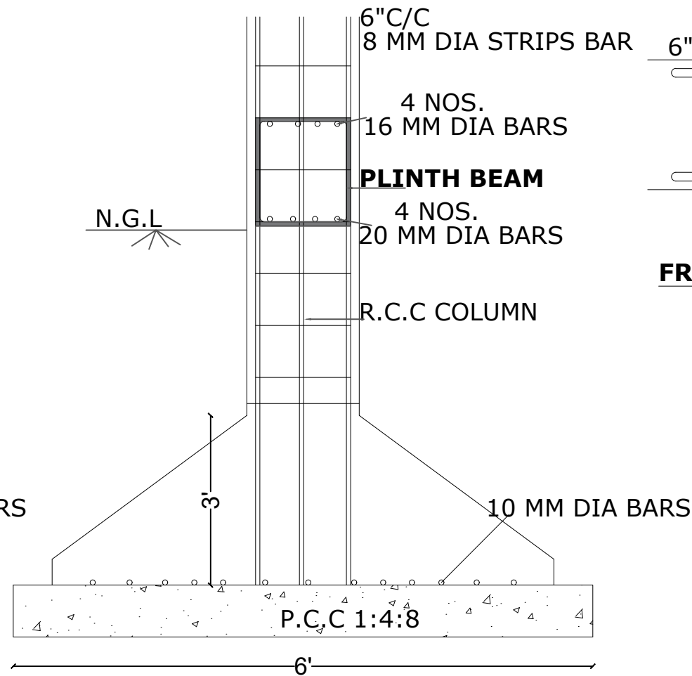
FOOTING DETAIL R.C.C COLUMN 12" X 12"
